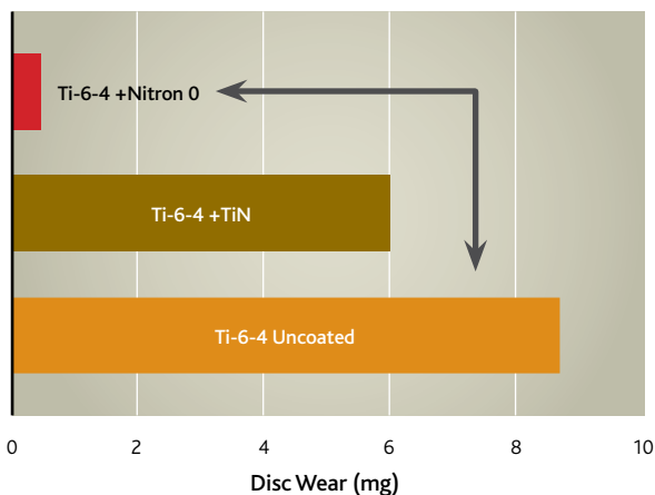
Sliding wear comparison of uncoated Ti-6-4 vs TiN coated and Nitron 0 coated
