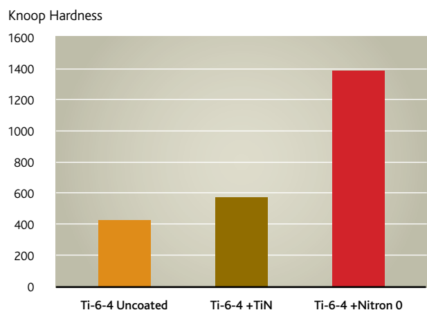
Knoop hardness values for 100g load (Titanium alloy uncoated/TiN coated/Nitron 0 coated)
